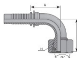
METRIC FEMALE 24° CONE - 90° ELBOW - L TYPE
