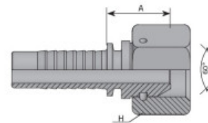
BSPP FEMALE (THRUST-WIRE NUT)
