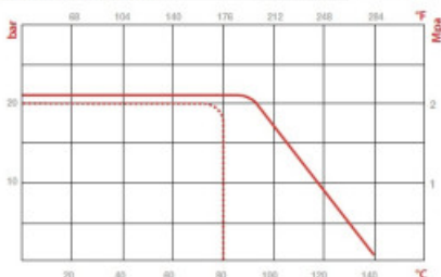
DIAGRAMMA PRESSIONE - TEMPERATURA PRESSURE - TEMPERATURE RATINGS DIAGRAM DRUCK - TEMPERATUR DIAGRAM
