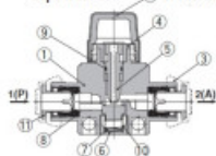
3-port valve: VHK3A series
