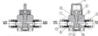
2-port valve: VHK2A series
