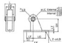
Pivot Bracket Standard: Double Acting Single Rod Series CM2
