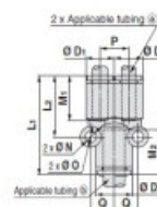
Different Diameter Union "Y": KQ2U
