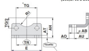
Dimensions: Mounting Brackets
